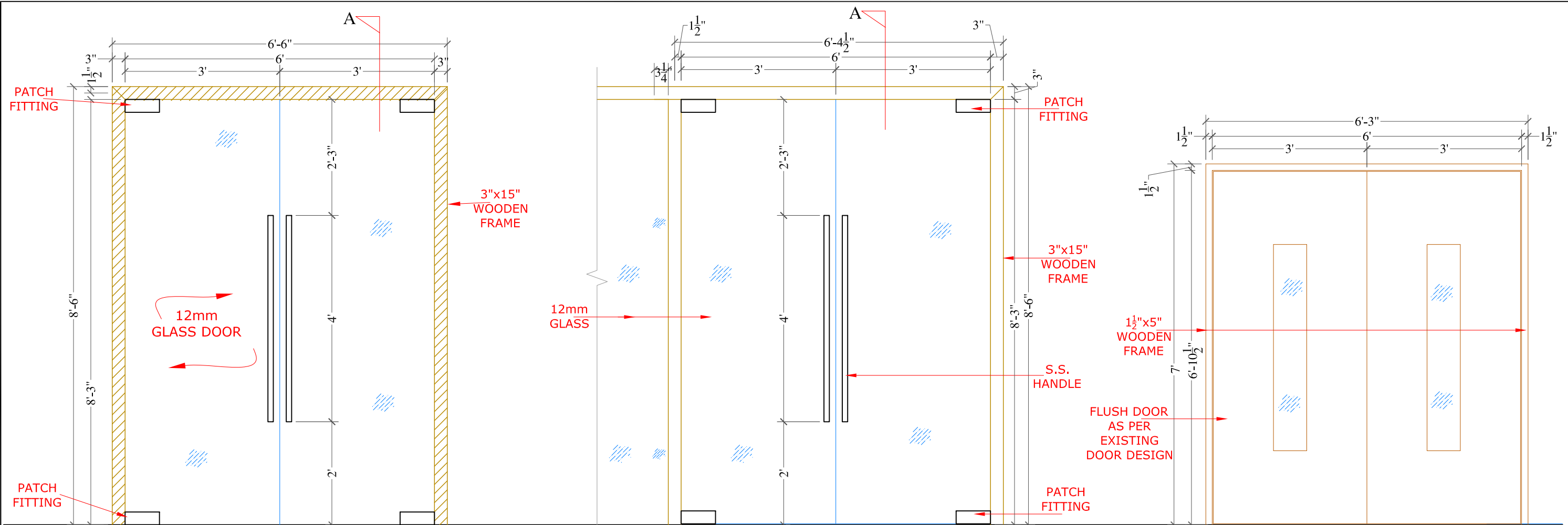
D1b#01 FLUSH DOOR (AS PER MANUFACTURER)
