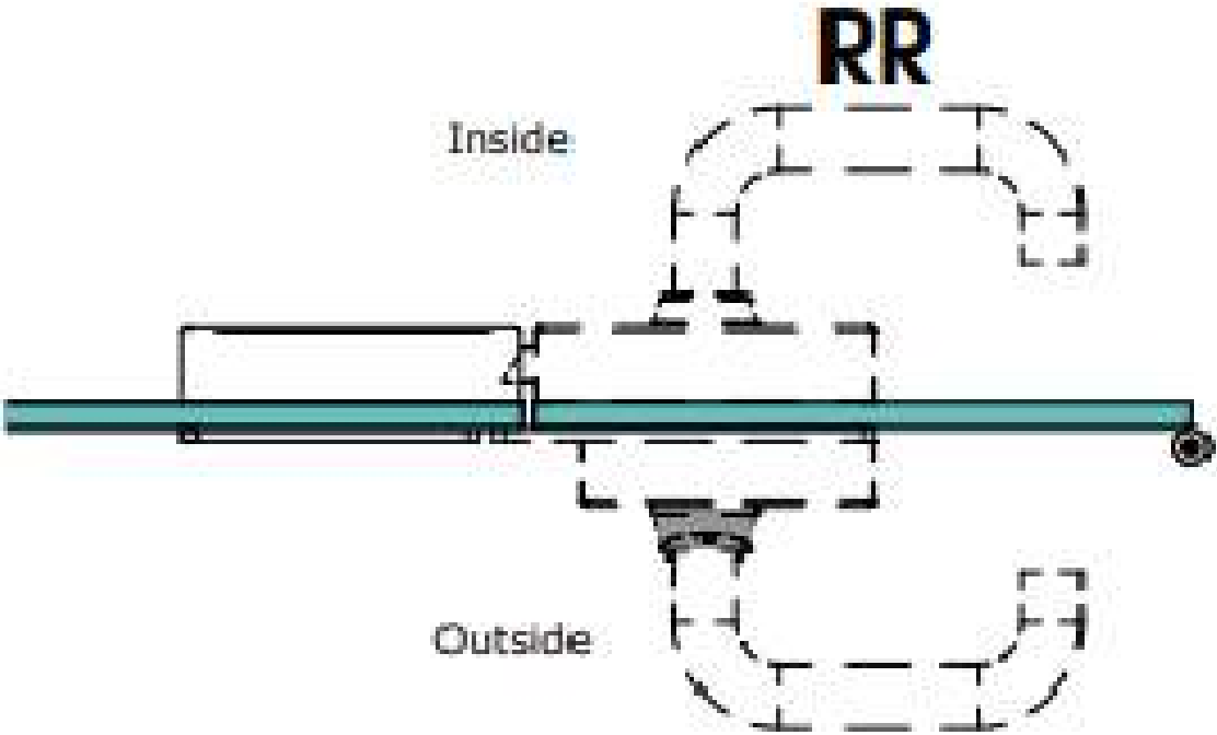
LOCK SYSTEM DETAIL FOR DOUBLE DOOR
