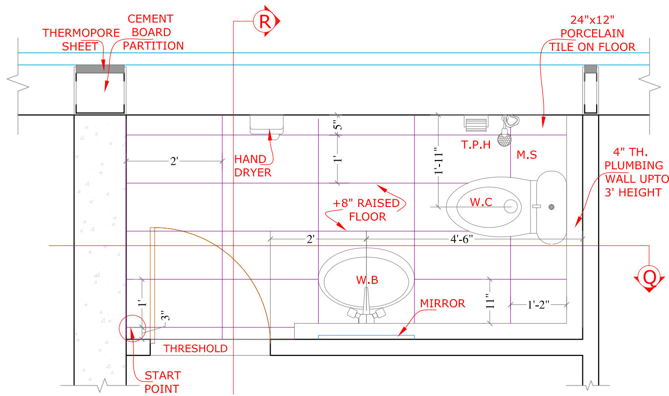
(VISITORS) TOILET-02, 9'-6"x4'-6" SCALE 1/2"=1'-0"
