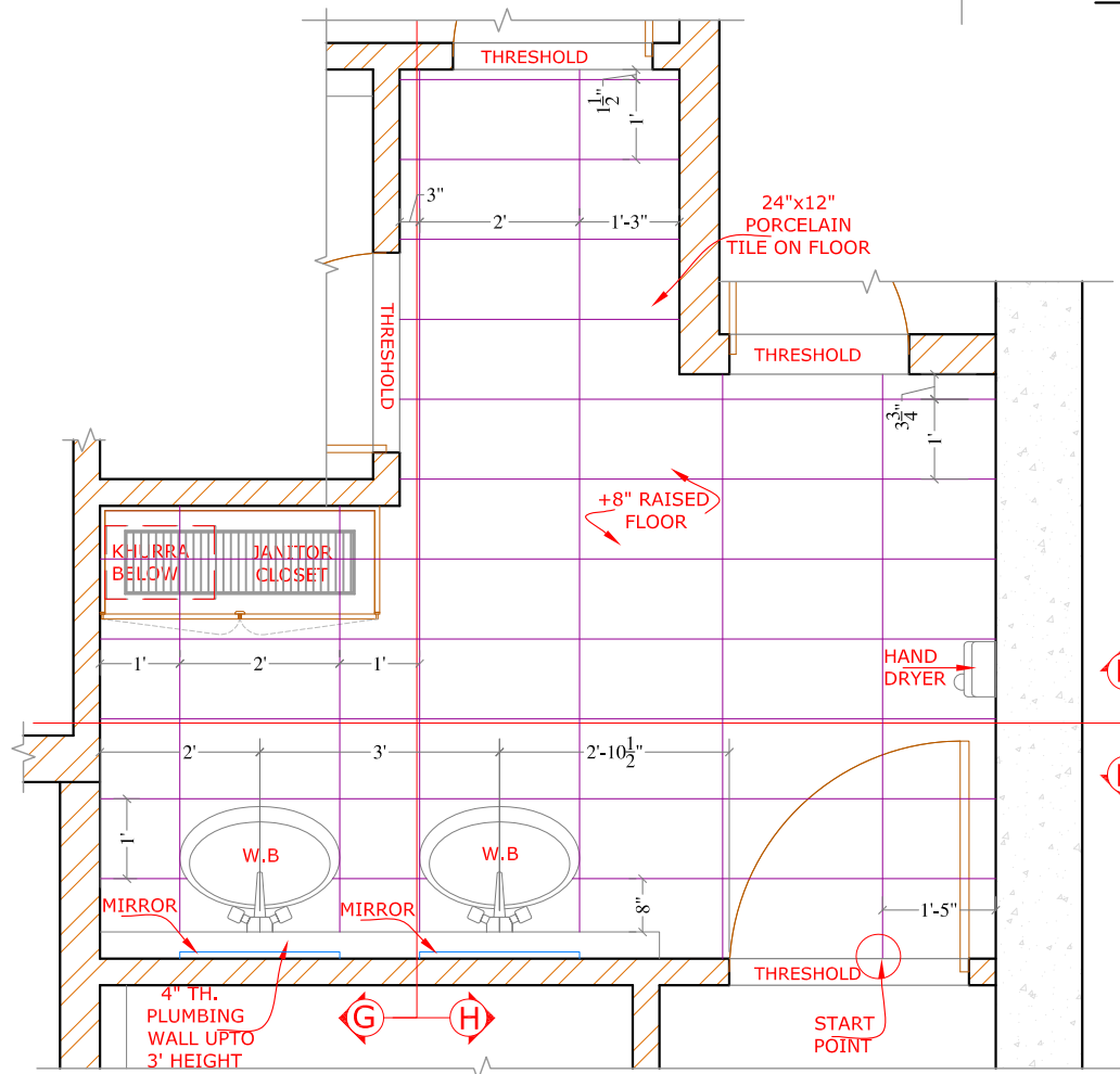
(GENTS).TOILE, 11'-21/2"x5'-6" SCALE 3/8"=1'-0"
