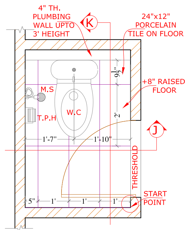
(GENTS) TOILET -01 3'-5"x5'-11 1/2" SCALE 1/2"=1'-0"
