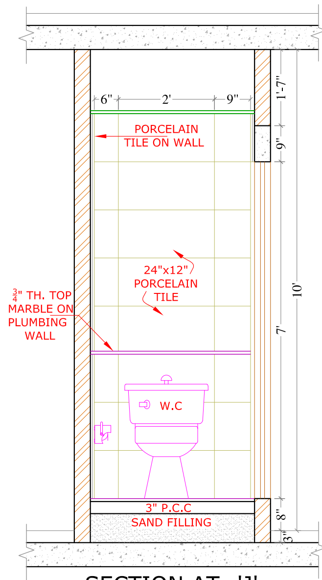
SECTION AT -'J' SCALE, \frac{1}{2} "=1'-0"
