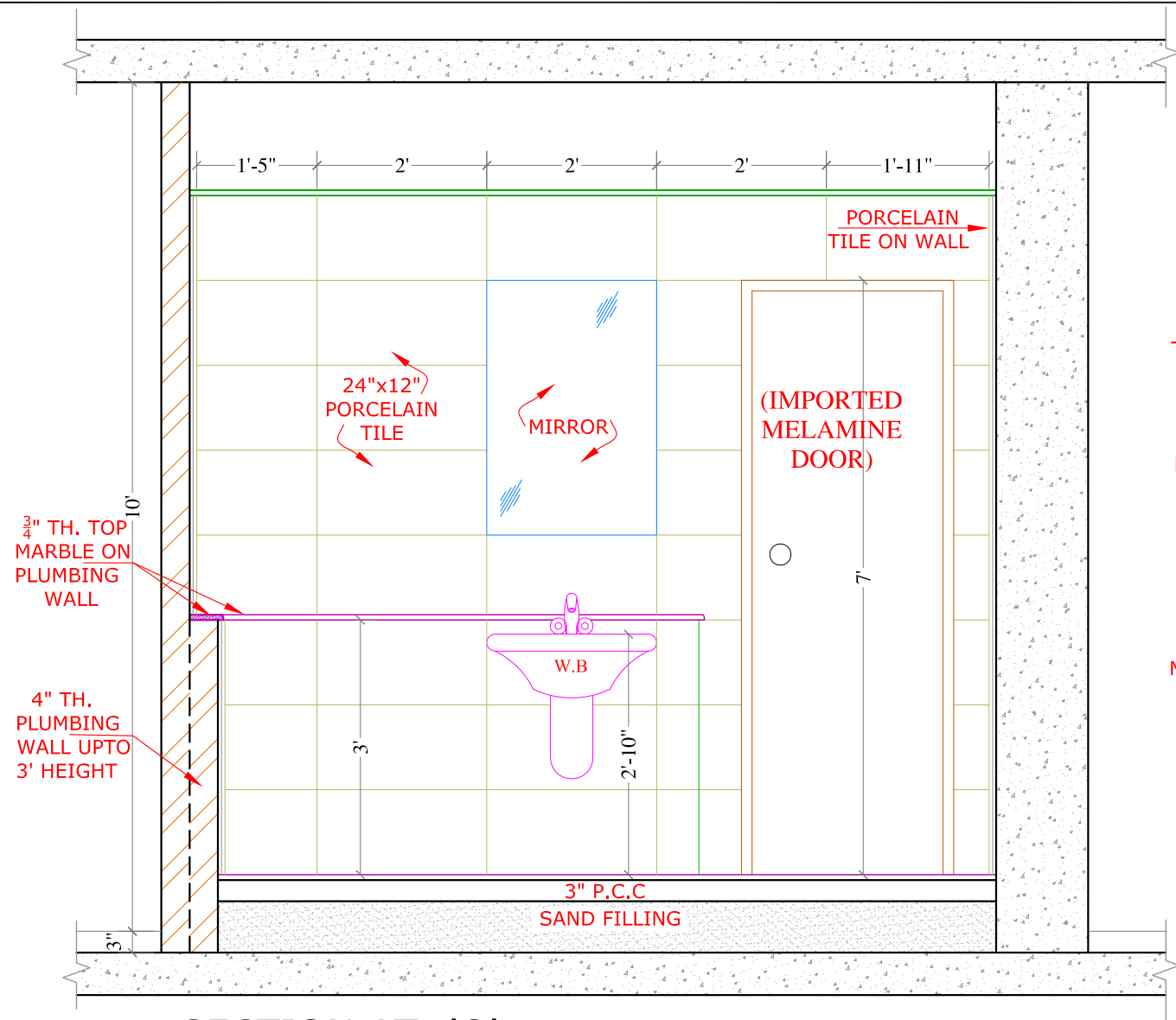
SECTION AT -'Q' SCALE, 1/2"=1'-0"
