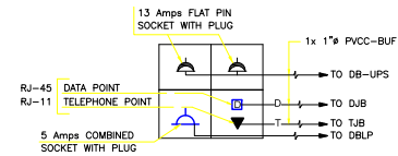
TENTATIVE DETAIL OF FLOOR OUTLET PLATE
