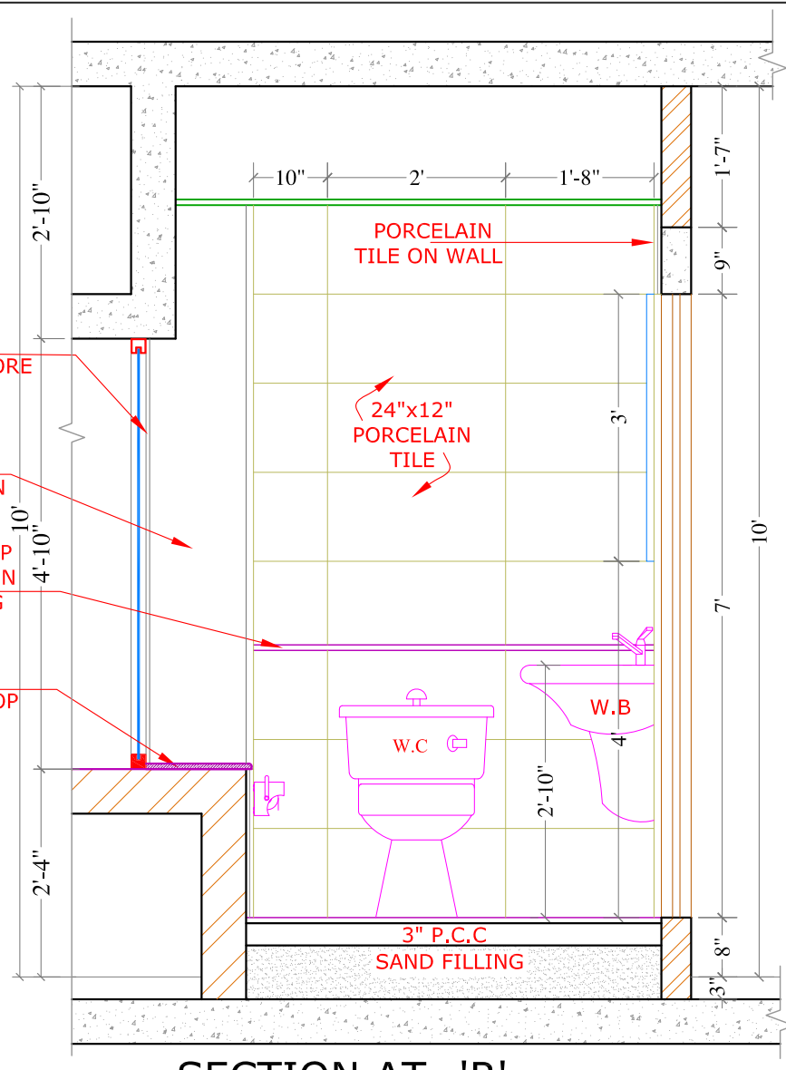
SECTION AT -'R' SCALE, 1/2"=1'-0"
