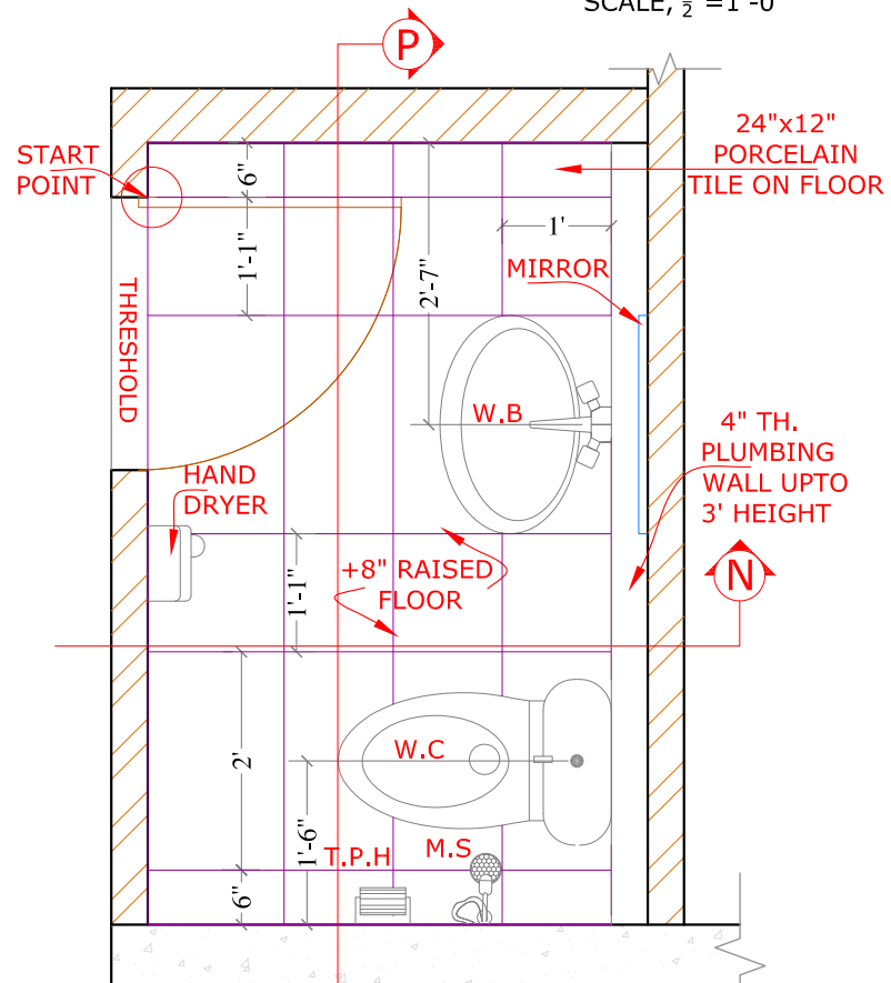
(VISITORS) TOILET-01, 4'-7"x7'-2"
