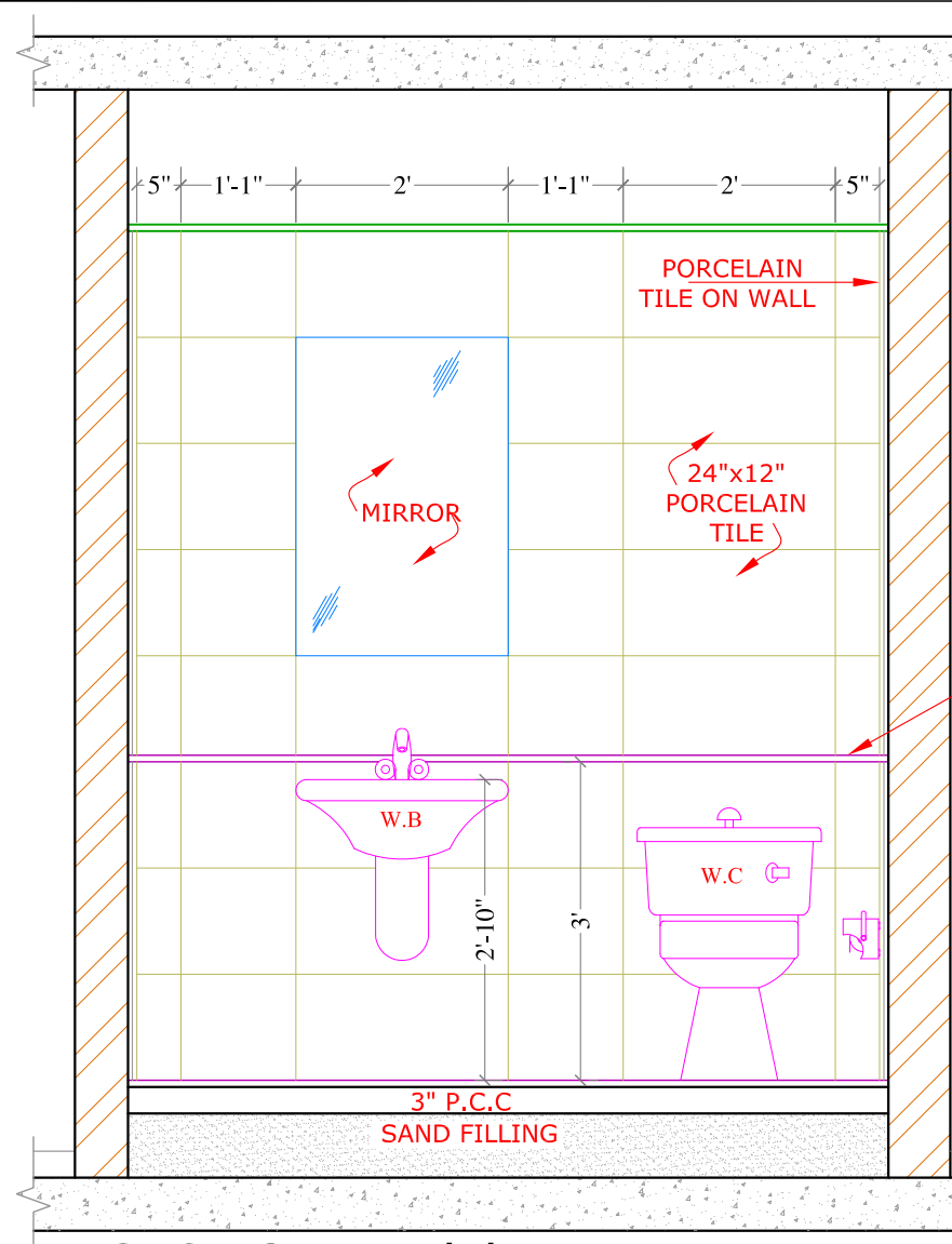
SECTION AT -'P'
