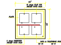
TENTATIVE DETAIL OF M.S FLOOR OUTLET BOX- (FOB)
