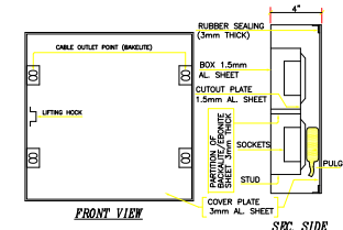
TENTATIVE DETAIL OF M.S FLOOR OUTLET BOX- (FOB)
