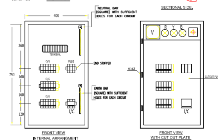
TENTATIVE CONSTRUCTIONAL DETAIL OF- DISTRIBUTION BOARD (FOR PRECESSED TYPE)
