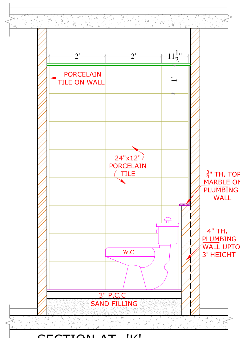
SECTION AT -'K' SCALE, \frac{1}{2} "=1'-0"
