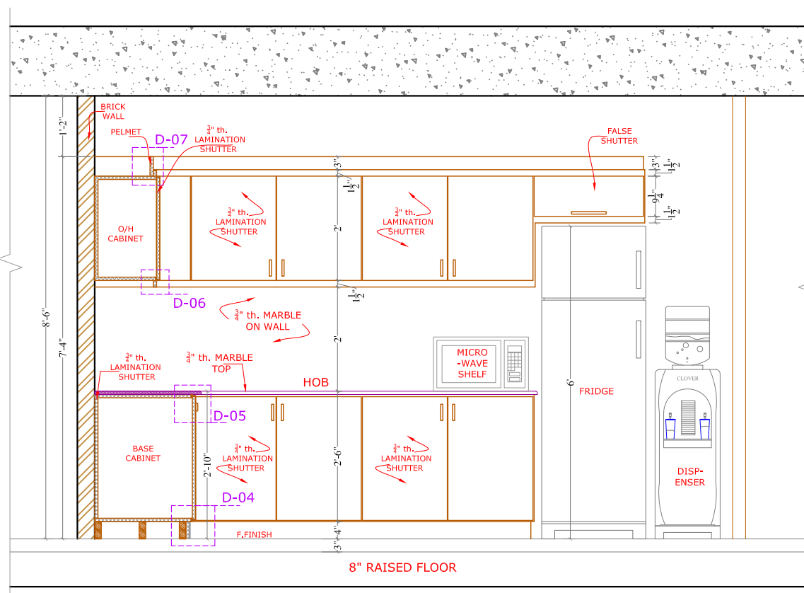
SECTION AT-A' SCALE, \frac{1}{2}"=1'-0"
