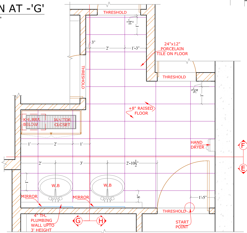
(GENTS).TOILE, 11'-21 1/2"x5'-6" SCALE 3/8"=1'-0"
