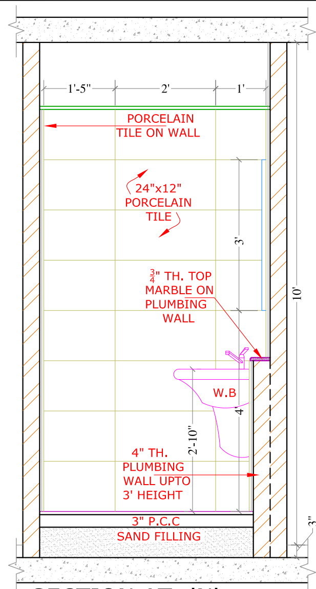
SECTION AT -'N'
