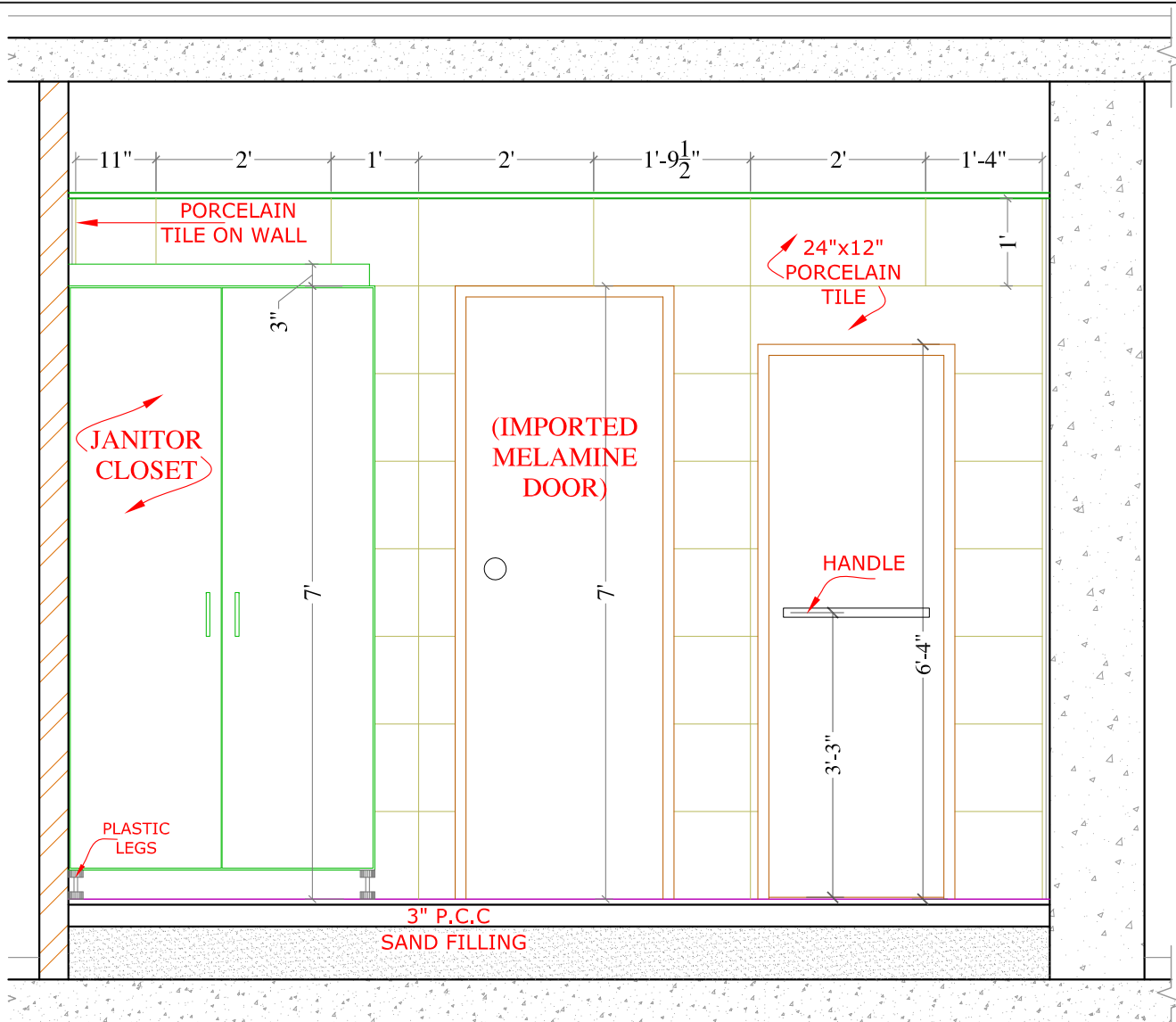
SECTION AT -'F' SCALE, 1/2"=1'-0"
