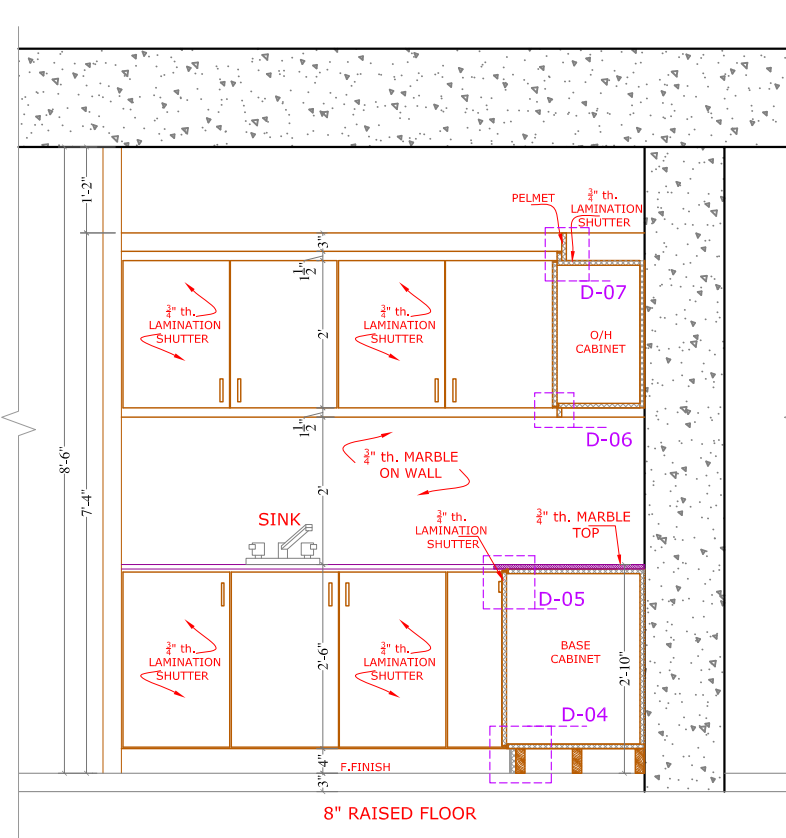
SECTION AT-B' SCALE, \frac{3}{8}"=1'-0"
