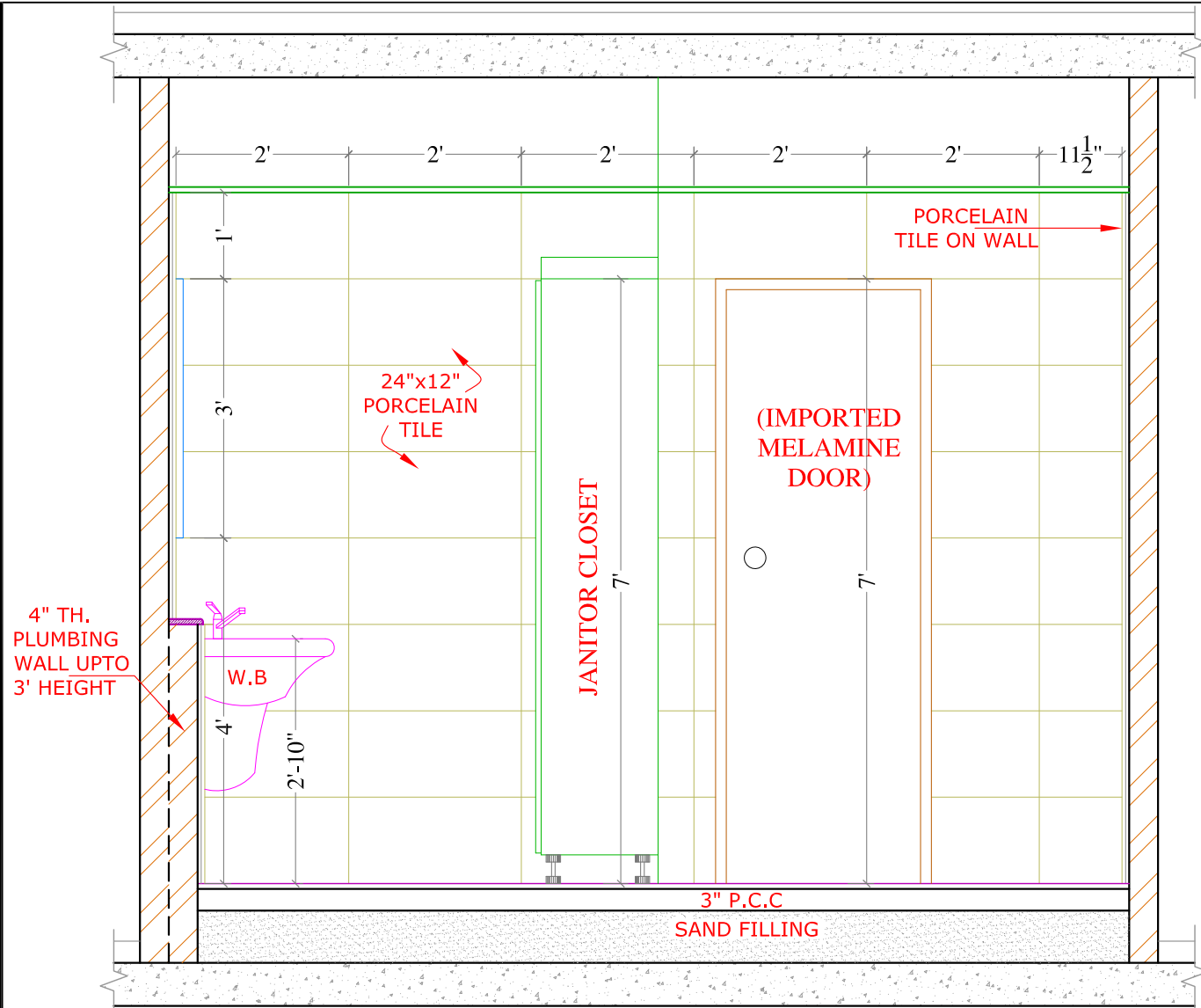
SECTION AT -'G' SCALE, 1/2"=1'-0"
