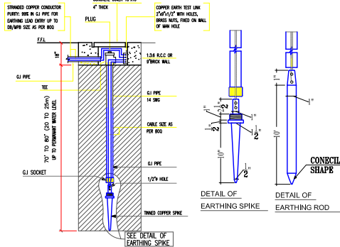
EARTHING DETAIL BORE TYPE
