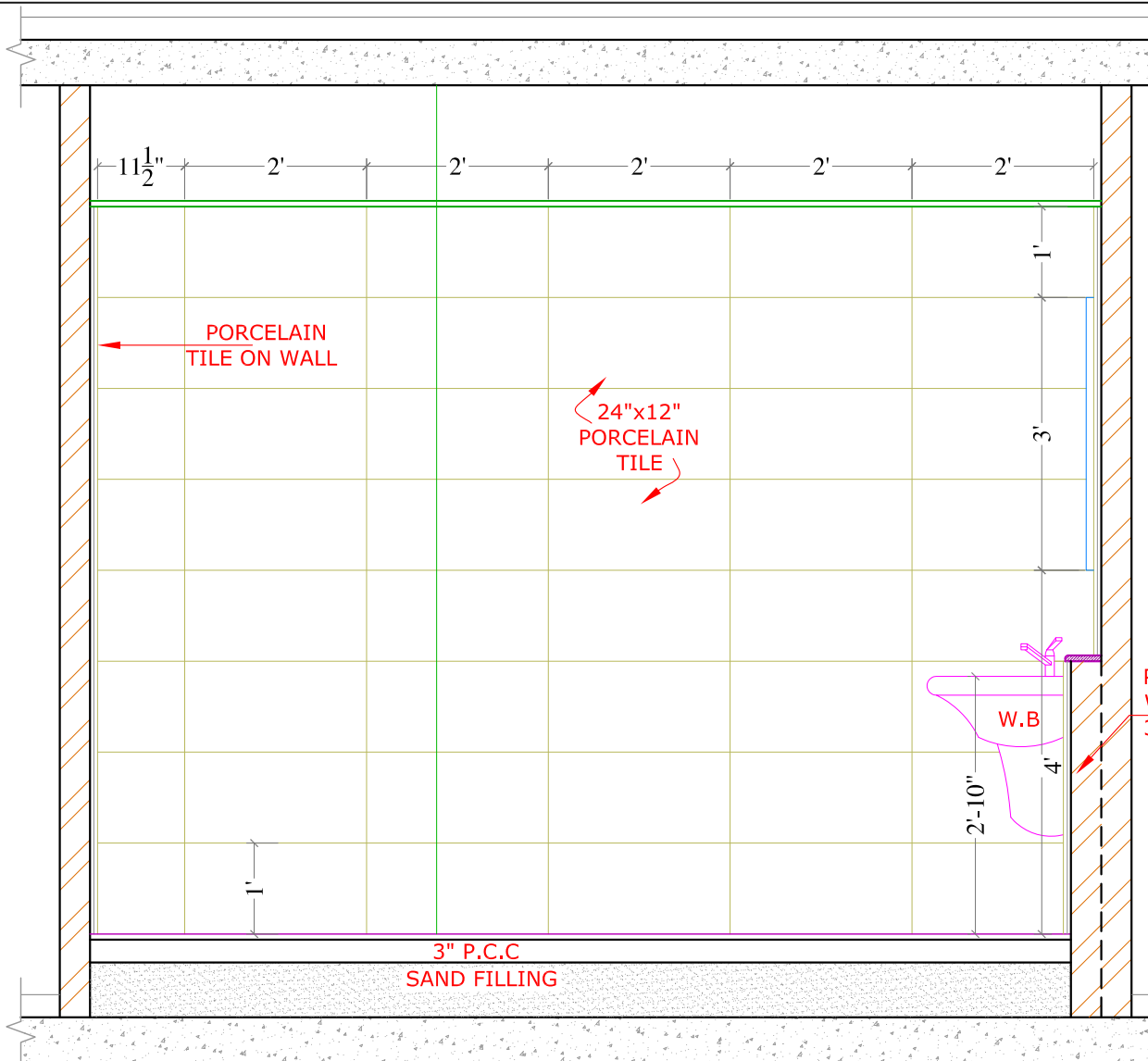
SECTION AT -'H' SCALE, 1/2"=1'-0"
