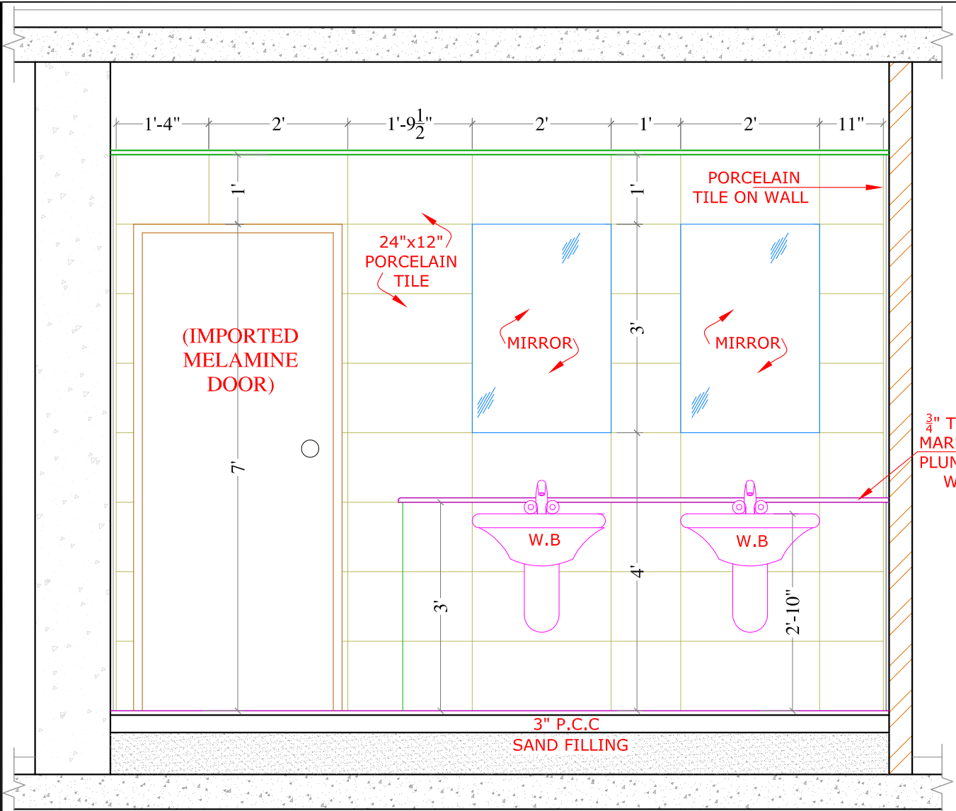
SECTION AT -'E' SCALE, 1/2"=1'-0"
